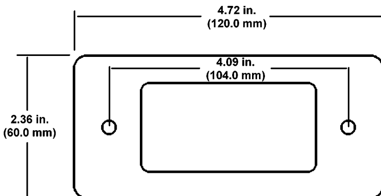
Mounting Frame P.N. 474630 (not to scale)
